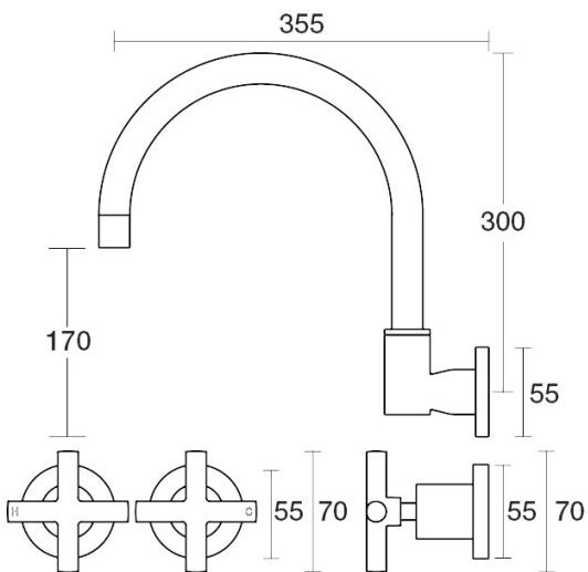
Portsea Spa Set XL Wall Swivel B29.064.1.34 - Matt Black
