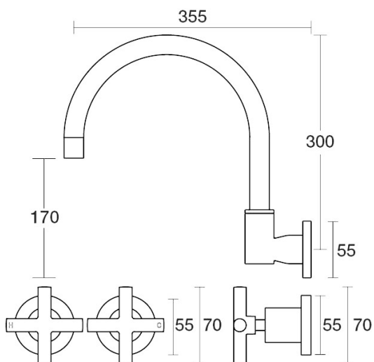
Portsea Spa Set XL Wall Swivel Ceramic Disc B29.064.2.23 - Gunmetal
