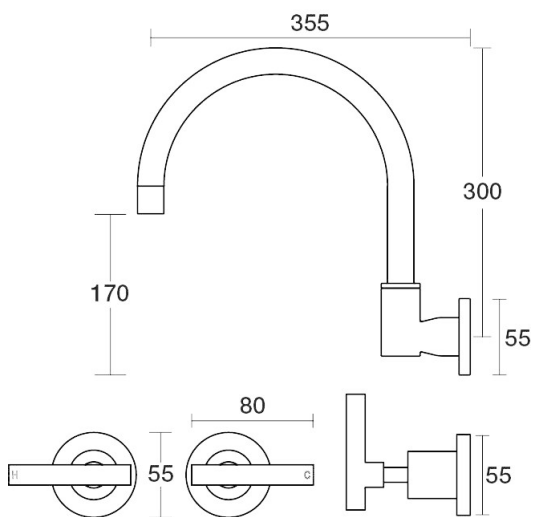
Portsea Spa Set XL Wall Swivel Lever Ceramic Disc 29.064.3.39 - Antique Bronze
