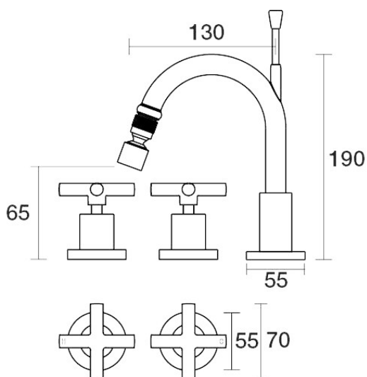
Portsea Bidet Set Fixed B29.071.1.11 - 23k Gold
