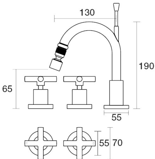
Portsea Bidet Set Fixed B29.071.1.52 - Burnished
