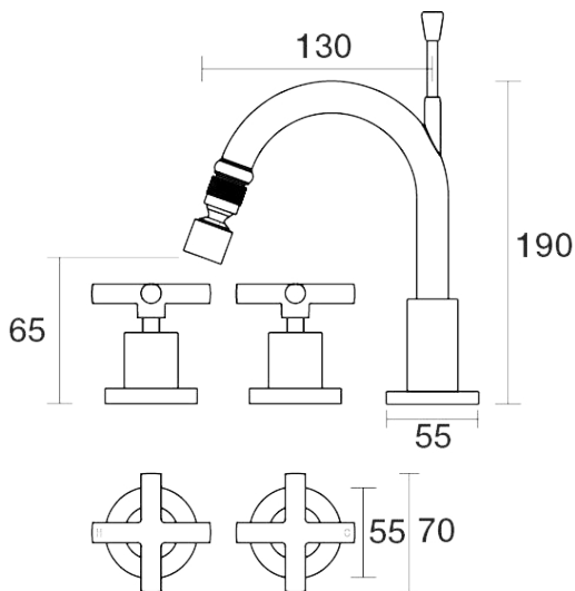
Portsea Bidet Set Fixed Ceramic Disc B29.071.2.01 - Chrome
