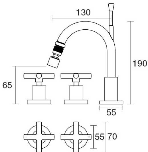
Portsea Bidet Set Fixed Ceramic Disc B29.071.2.44 - Antique Copper
