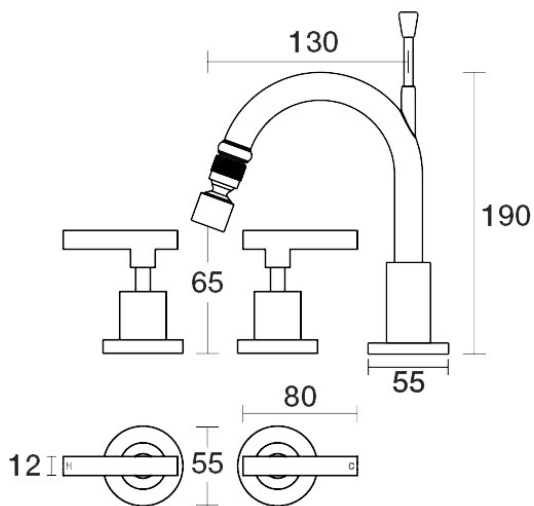
Portsea Bidet Set Fixed Lever Ceramic Disc B29.071.3.54 - Volcanic Grey
