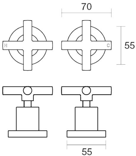
Portsea Top Assemblies Wall Pair B29.082.1.01 - Chrome
