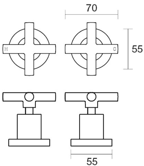
Portsea Top Assemblies Wall Pair Ceramic Disc B29.082.2.02 - Brushed Chrome
