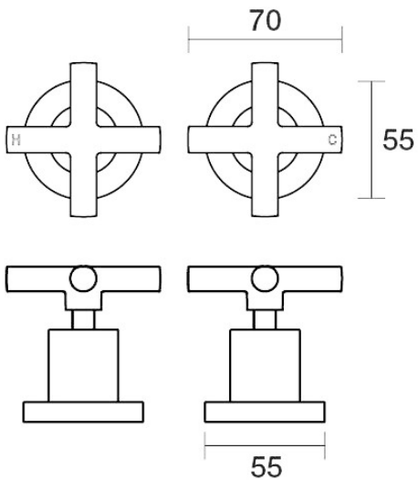
Portsea Top Assemblies Wall Pair Ceramic Disc B29.082.2.24 - Brushed Gunmetal
