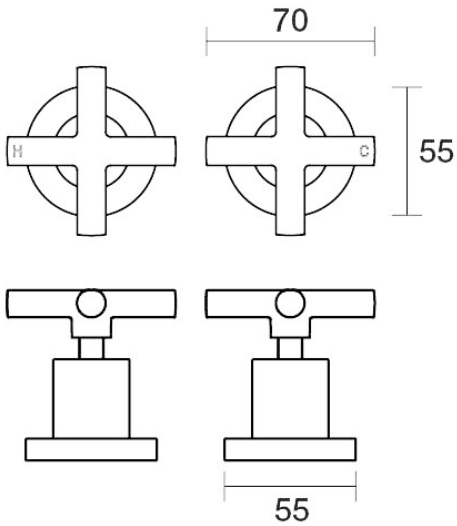
Portsea Top Assemblies Wall Pair Ceramic Disc B29.082.2.34 - Matt Black
