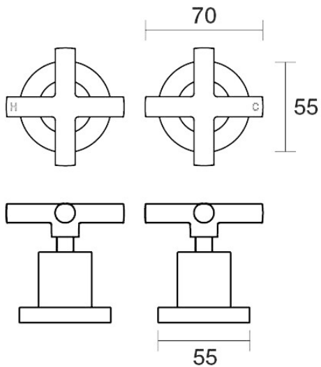
Portsea Top Assemblies Wall Pair Ceramic Disc B29.082.2.43 - Brass
