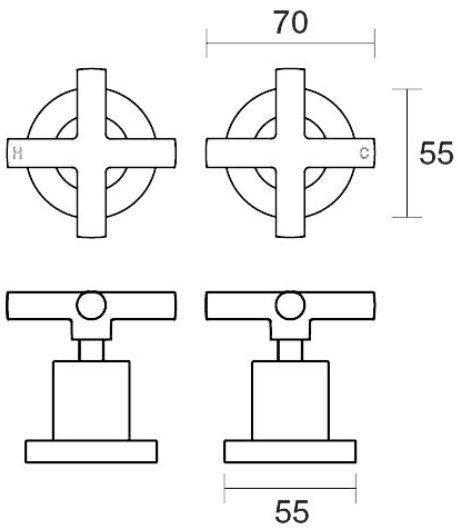
Portsea Top Assemblies Wall Pair Ceramic Disc B29.082.2.57 - Matt Nickel
