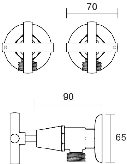
Portsea Washing Machine Stops Wall Pair B29.091.1.43 - Brass
