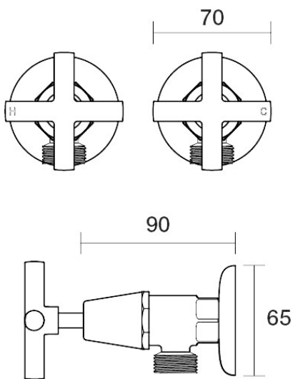
Portsea Washing Machine Stops Wall Pair B29.091.1.45 - Native Brass
