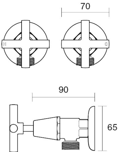
Portsea Washing Machine Stops Wall Pair B29.091.1.67 - Vintage Brass
