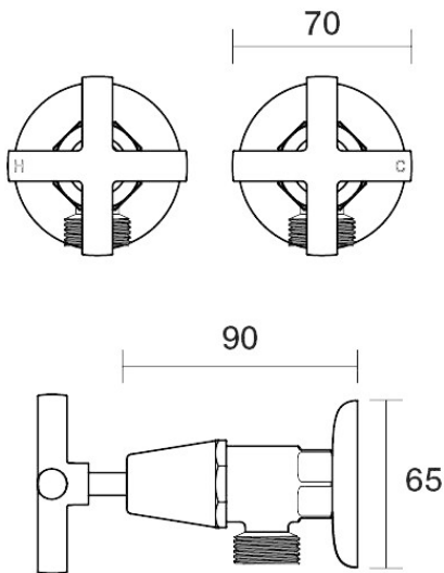
Portsea Washing Machine Stops Wall Pair Ceramic Disc B29.091.2.41 - Brushed Brass
