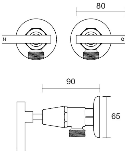
Portsea Washing Machine Stops Wall Pair Lever Ceramic Disc B29.091.3.39 - Antique Bronze
