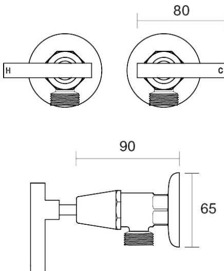
Portsea Washing Machine Stops Wall Pair Lever Ceramic Disc B29.091.3.41 - Brushed Brass
