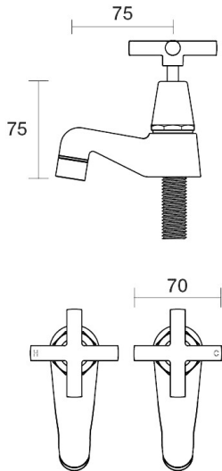
Portsea Pillar Taps Pair B29.111.1.54 - Volcanic Grey
