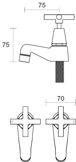
Portsea Pillar Taps Pair Ceramic Disc B29.111.2.40 - Rumbled Brass
