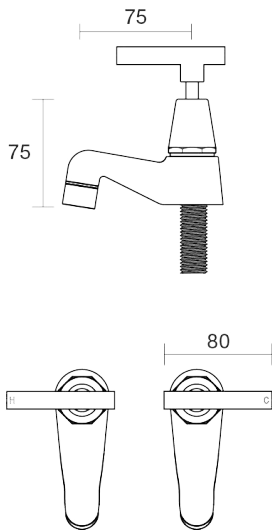
Portsea Pillar Taps Pair Lever Ceramic Disc B29.111.3.01 - Chrome
