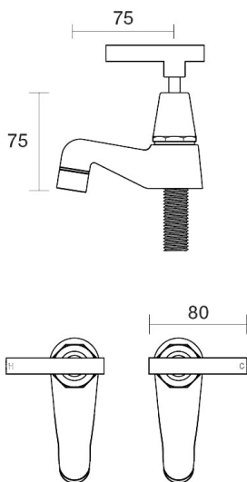
Portsea Pillar Taps Pair Lever Ceramic Disc B29.111.3.45 - Native Brass
