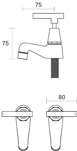
Portsea Pillar Taps Pair Lever Ceramic Disc B29.111.3.52 - Burnished
