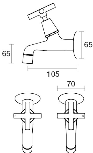
Portsea Female Bibs Wall Pair B29.121.1.32 - Midnight Black
