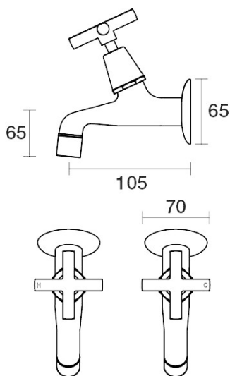
Portsea Female Bibs Wall Pair B29.121.1.57 - Matt Nickel
