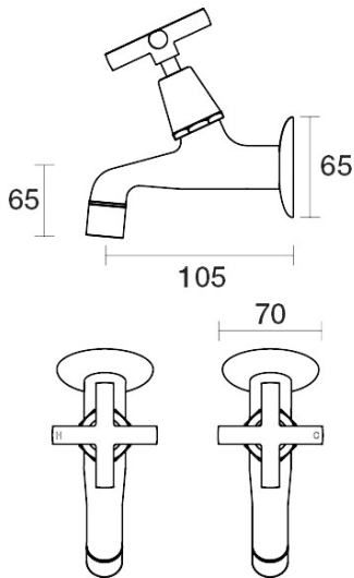
Portsea Female Bibs Wall Pair Ceramic Disc B29.121.2.52 - Burnished
