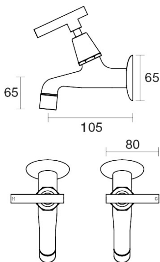
Portsea Female Bibs Wall Pair Lever Ceramic Disc B29.121.3.11 - 23k Gold
