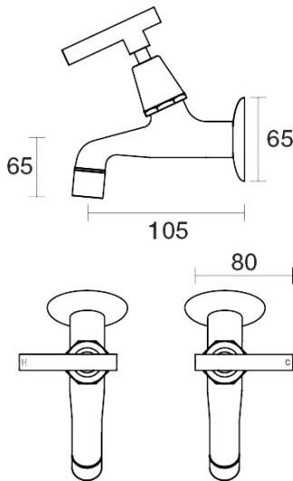
Portsea Female Bibs Wall Pair Lever Ceramic Disc B29.121.3.42 - Brushed Copper
