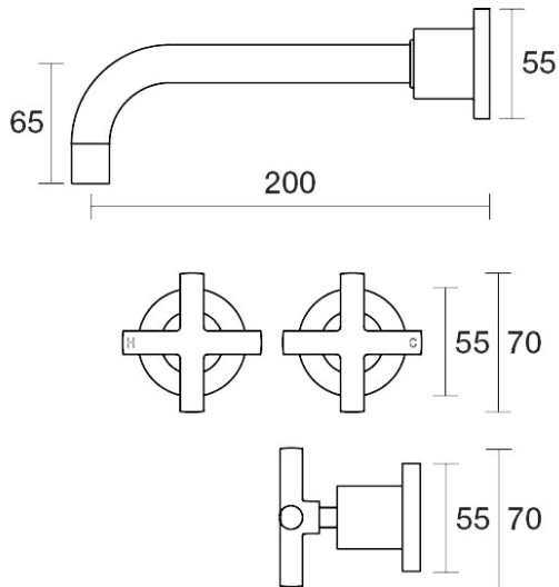
Portsea Wall Basin Set 200mm Outlet B29.152.1.44 - Antique Copper
