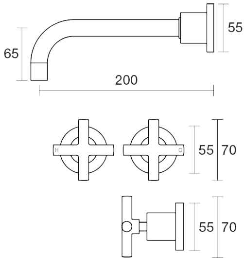
Portsea Wall Basin Set 200mm Outlet Ceramic Disc B29.152.2.01 - Chrome
