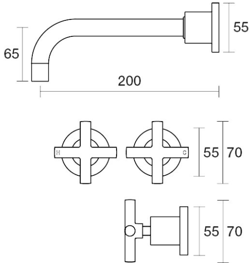
Portsea Wall Basin Set 200mm Outlet Ceramic Disc B29.152.2.26 - Black Sapphire
