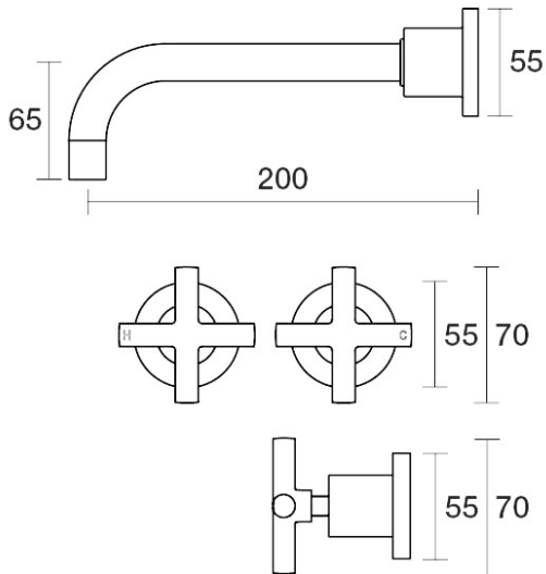
Portsea Wall Basin Set 200mm Outlet Ceramic Disc B29.152.2.39 - Antique Bronze
