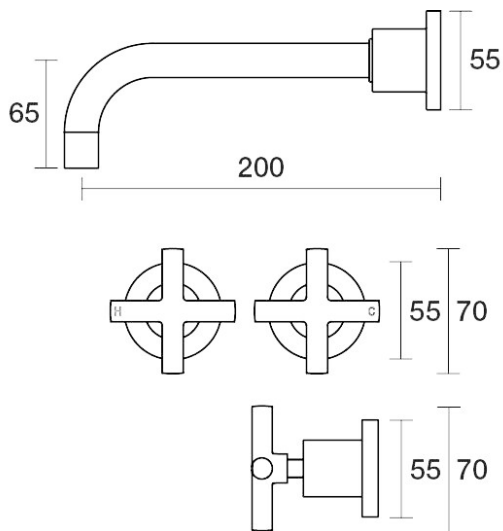
Portsea Wall Basin Set 200mm Outlet Ceramic Disc B29.152.2.45 - Native Brass
