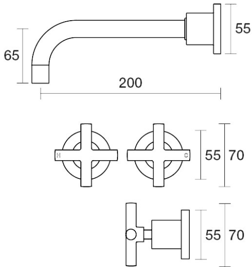
Portsea Wall Basin Set 200mm Outlet Ceramic Disc B29.152.2.52 - Burnished
