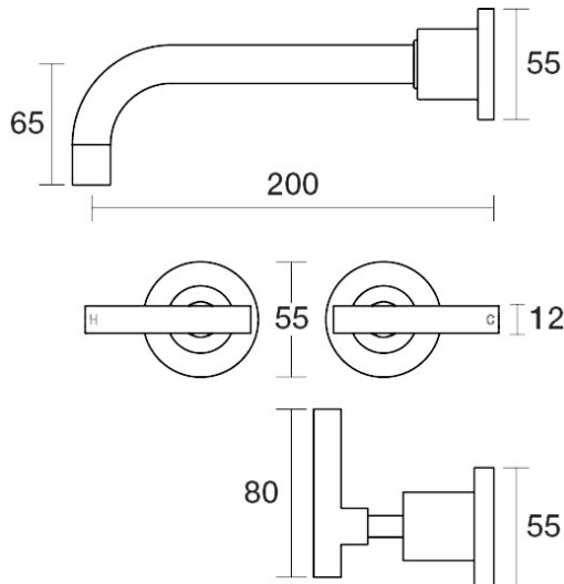
Portsea Wall Basin Set 200mm Outlet Lever Ceramic Disc B29.152.3.11 - 23k Gold
