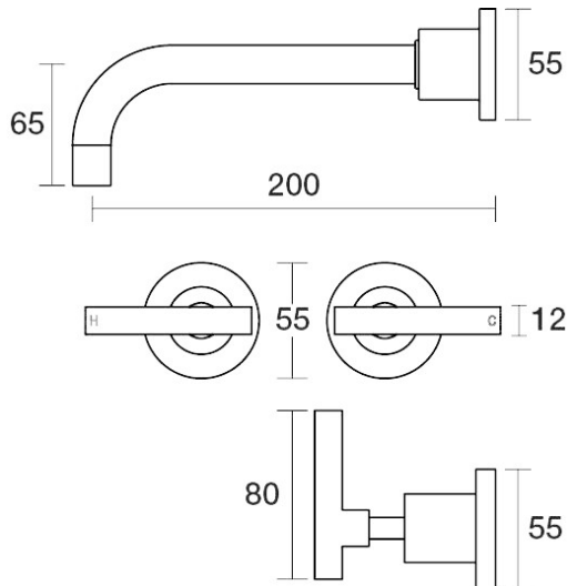
Portsea Wall Basin Set 200mm Outlet Lever Ceramic Disc B29.152.3.43 - Brass
