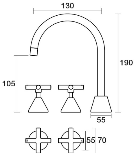
Poem Basin Set Swivel B30.011.1.23 - Gunmetal
