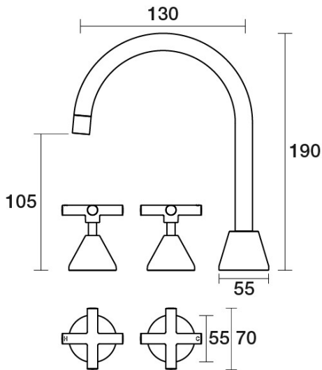
Poem Basin Set Swivel B30.011.1.34 - Matt Black
