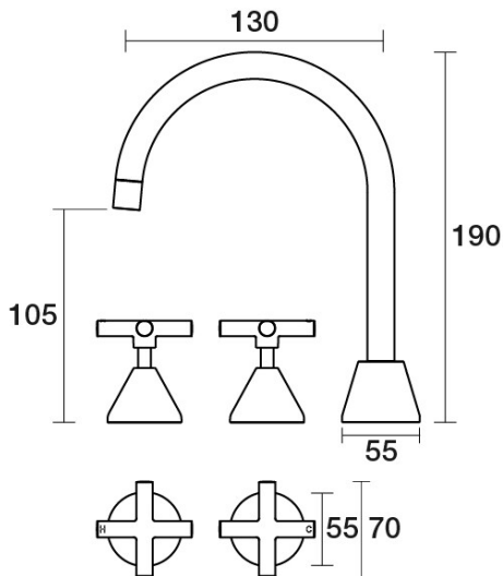
Poem Basin Set Swivel Ceramic Disc B30.011.2.02 - Brushed Chrome
