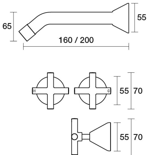
Poem Wall Bath Set 160mm Outlet B30.021.1.24 - Brushed Gunmetal
