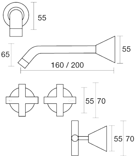
Poem Wall Bath Set 200mm Outlet B30.022.1.01 - Chrome
