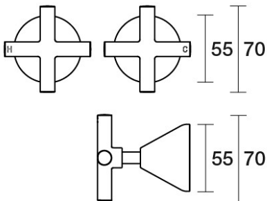
Poem Wall Bath Set 200mm Outlet Ceramic Disc B30.022.2.43 - Brass
