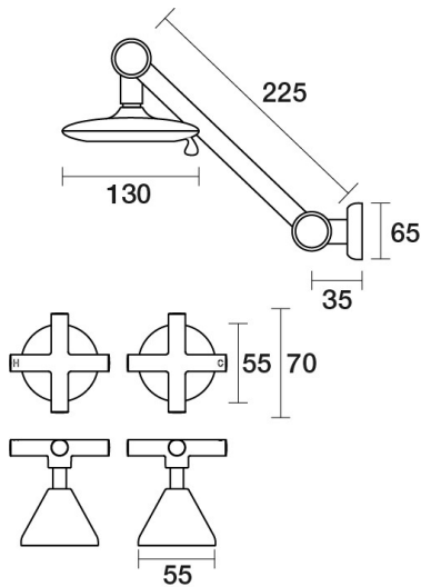
Poem Shower Set Adjustable Arm B30.031.1.19 - 23k Brushed Brass Gold
