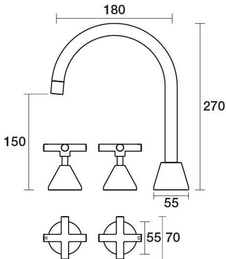
Poem Sink Set Hob Swivel Ceramic Disc B30.051.2.19 - 23k Brushed Brass Gold
