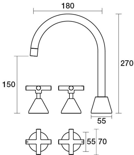
Poem Sink Set Hob Swivel Ceramic Disc B30.051.2.68 - Autumn Bronze
