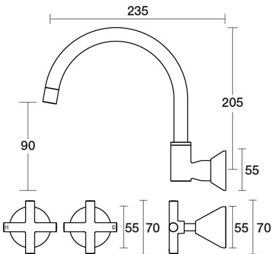
Poem Sink Set Wall Swivel B30.052.1.26 - Black Sapphire
