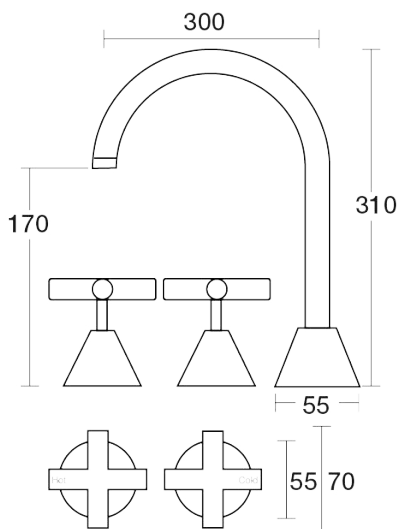
Poem Sink Set XL Hob Swivel Ceramic Disc B30.053.2.01 - Chrome
