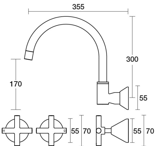
Poem Sink Set XL Wall Swivel B30.054.1.41 - Brushed Brass
